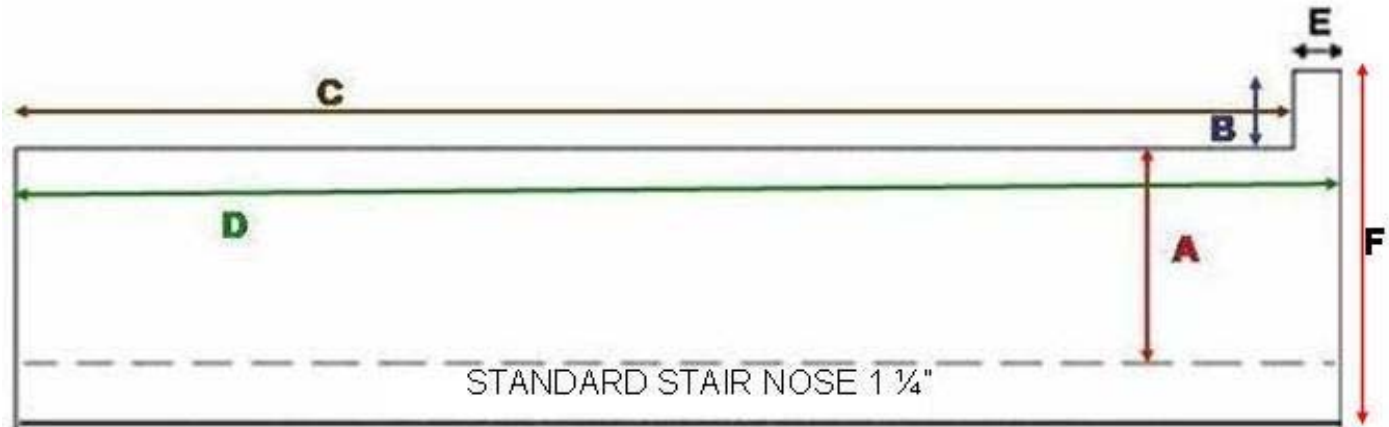
BELOW = TOP VIEW OF RIGHT HAND MITERED RETURN
